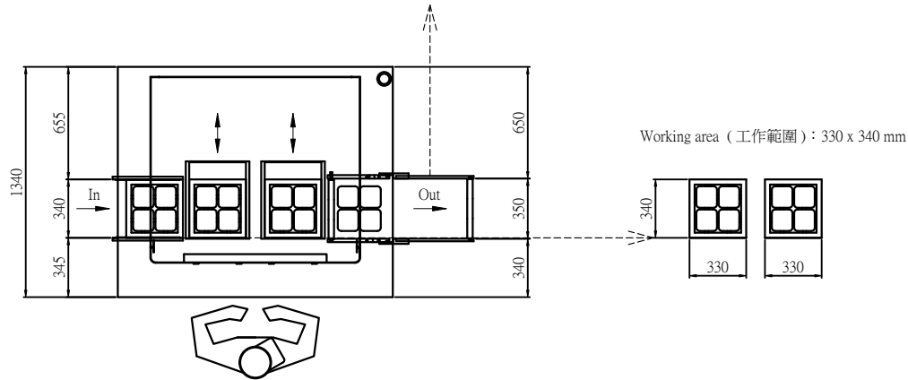
Flat oblique belt (平斜皮帶式) Standard (標準)
